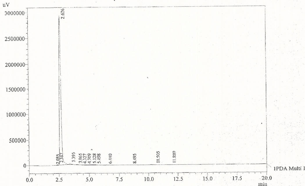
Chromatogram L-Abrine ID: \promonence\Data\2012JUNE-2012\0106121.lcd
